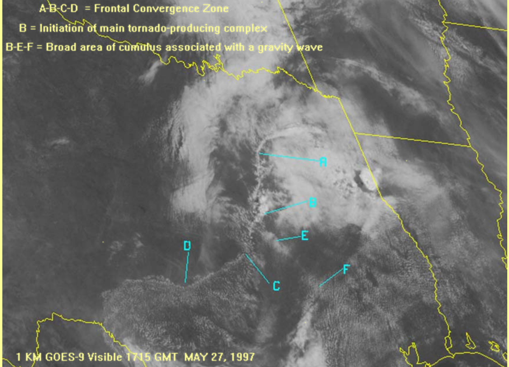
GOES-West view of organized cumulus convection along convergence zone ABCD, with convection being triggered at B by gravity wave EF
