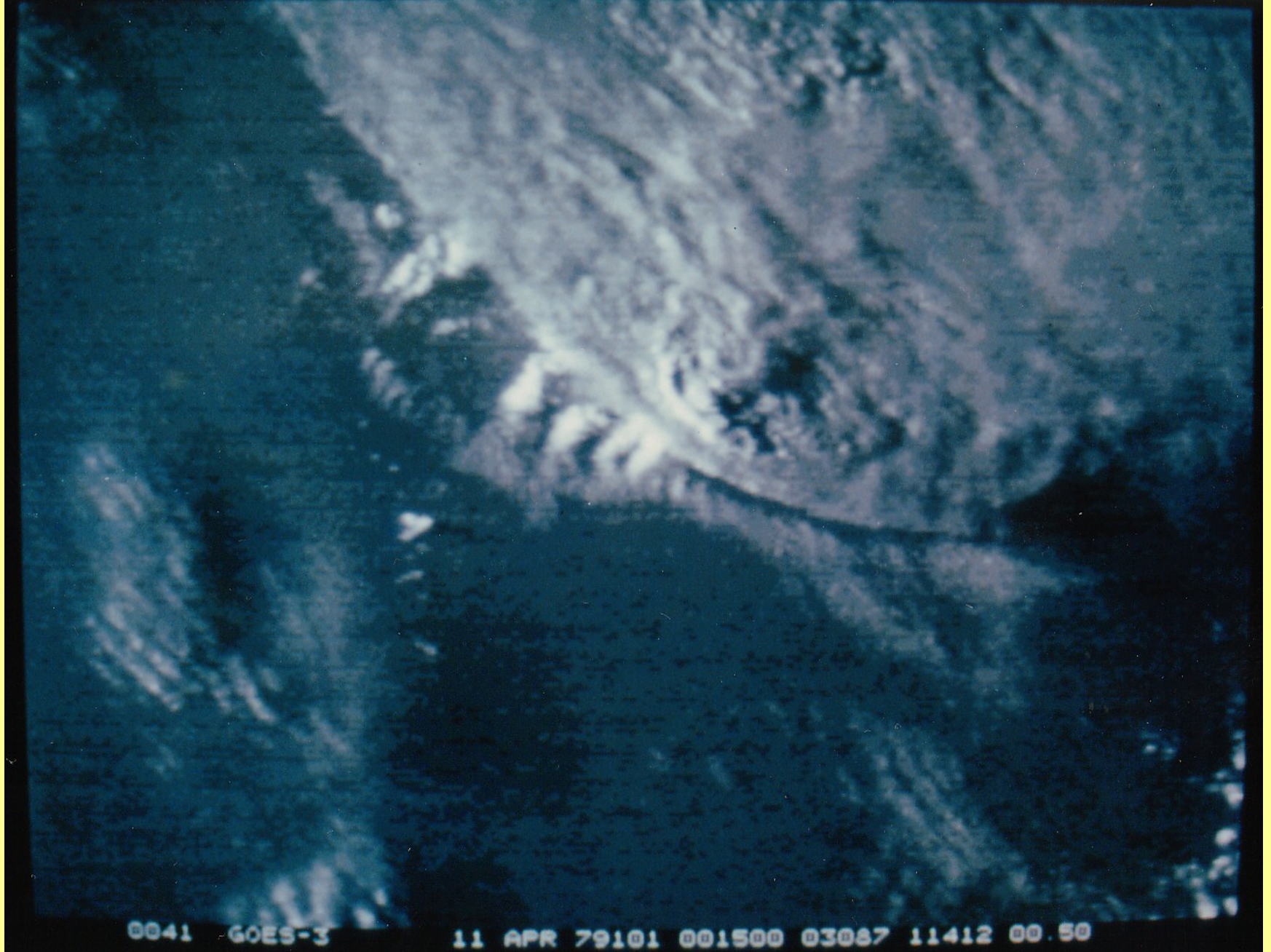
Wichita Falls, TX tornadic storm at 0015 GMT, Apr 11, '79
