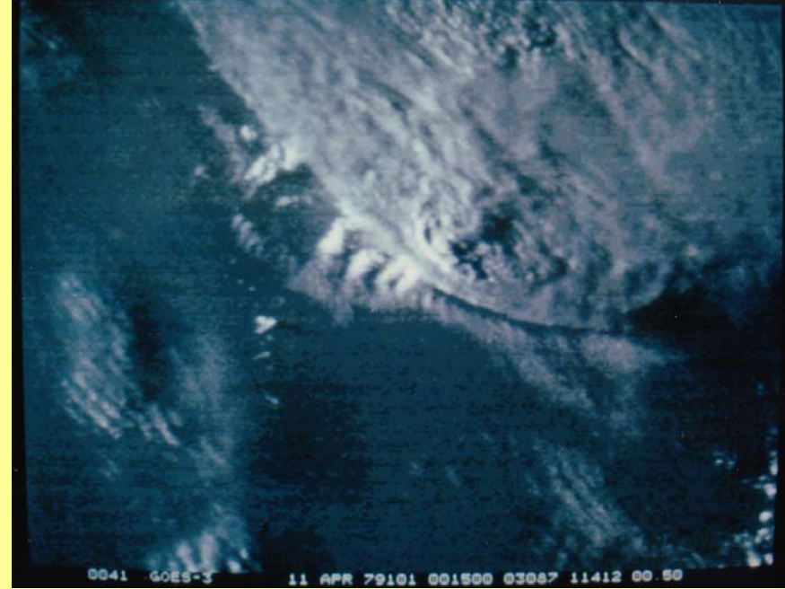
Wichita Falls, TX tornadic storm, 30 minutes later
