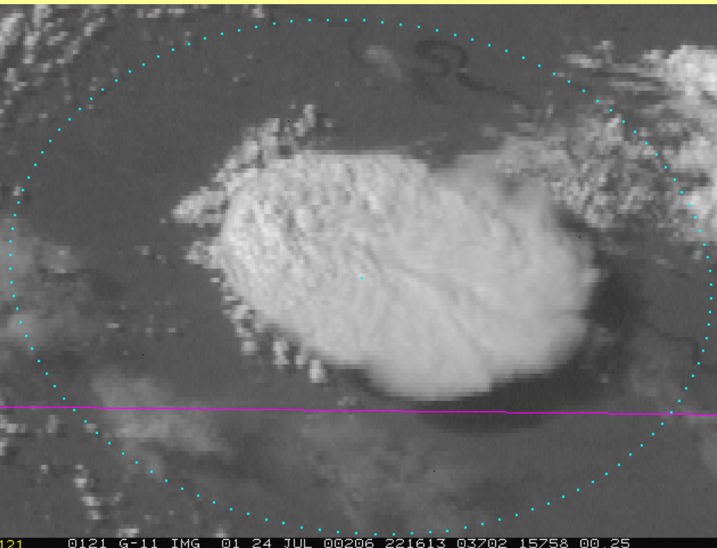
Figure 14. Early (top) and mature (bottom) stages of super-cell's life..
