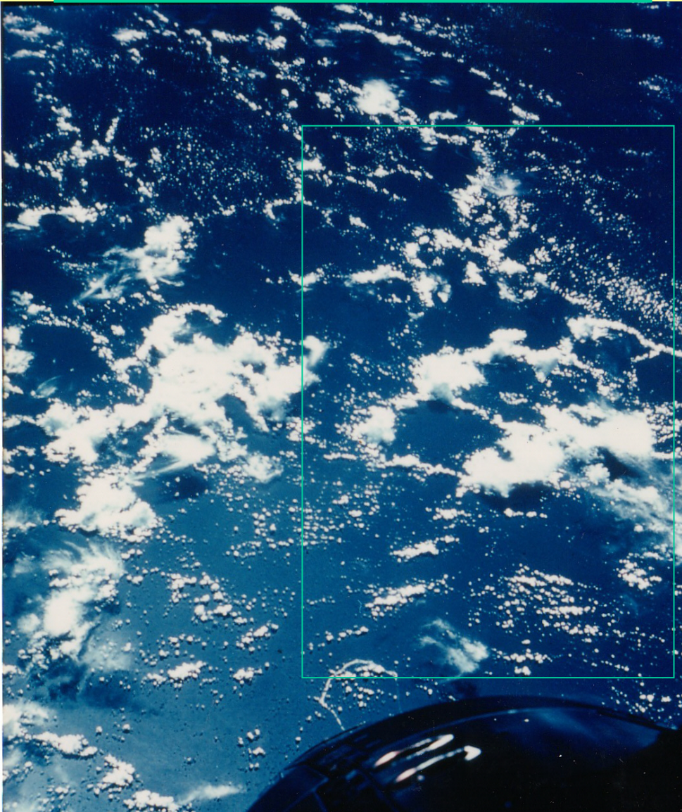
Photo from manned space craft
