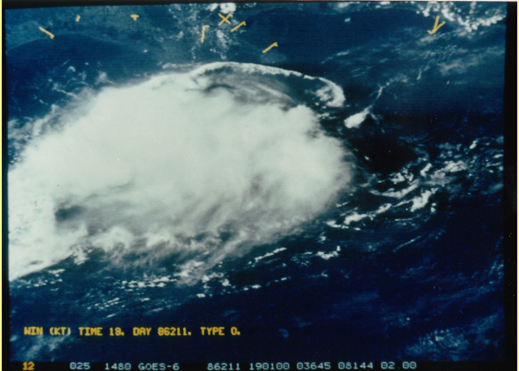
Arc cloud line moving northward from a large convective region over the Gulf of Mexico
