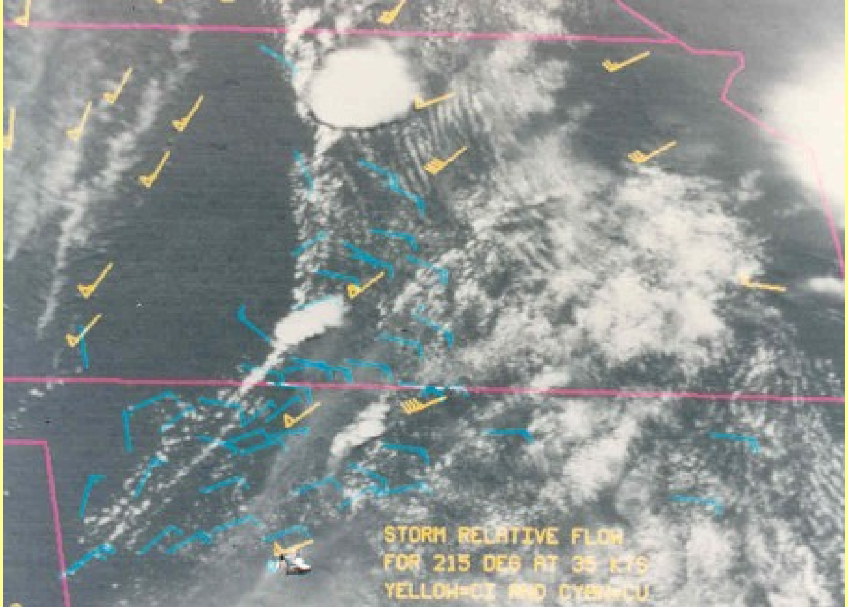
Thunderstorms developing along a cold front. Note the organization of the developing squall line as well as the cloud field ahead of it.
