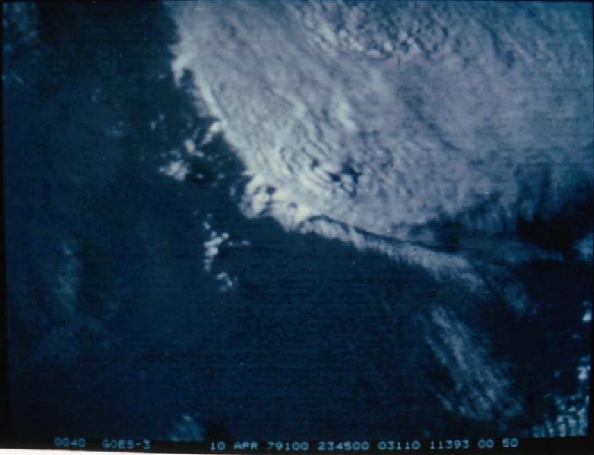
Wichita Falls, TX tornadic storm at 2345 GMT, Apr 10, '79
