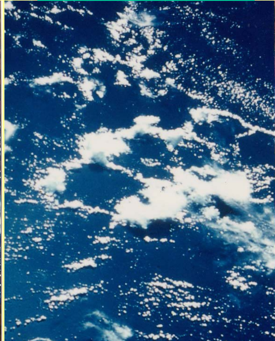
Expansion of inset to right
