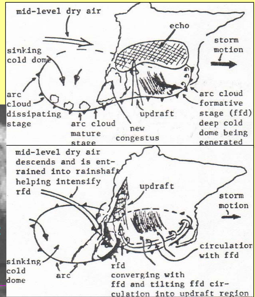
Figure 14. Early (top) and mature (bottom) stages of super-cell's life..
