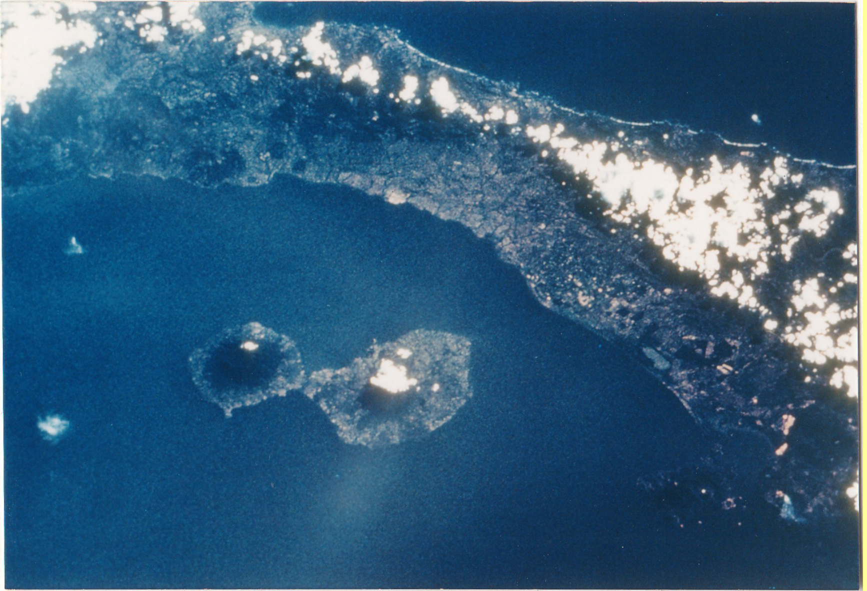
Example of mountain effect on convective development. Note the cumulus over the peaks and compensating subsidence areas.
