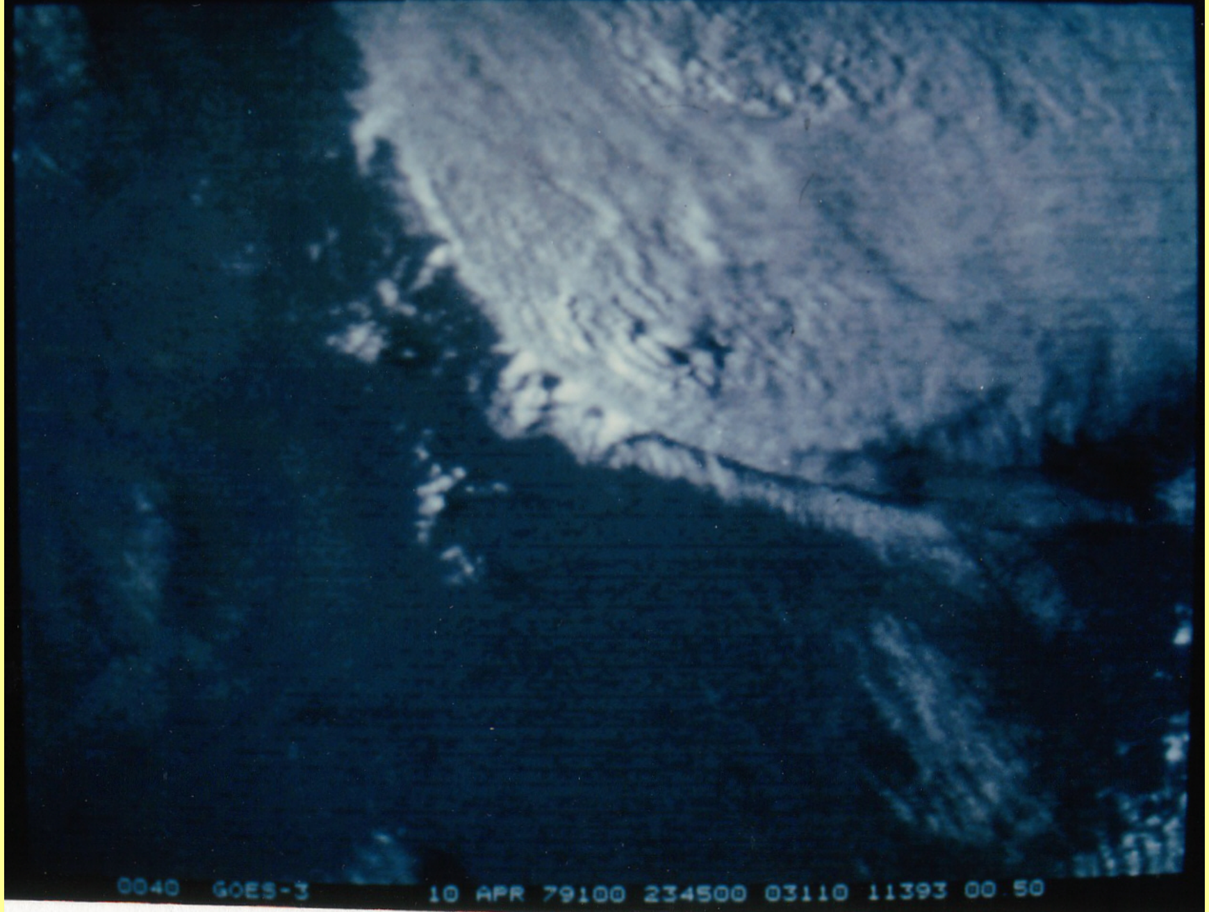
Wichita Falls, TX tornadic storm at 2345 GMT, Apr 10, '79
